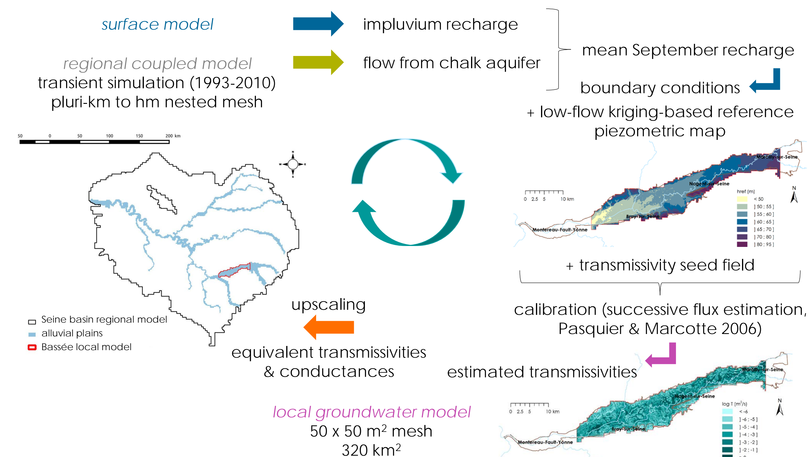
Fig. 6 – Multiscale modelling strategy
