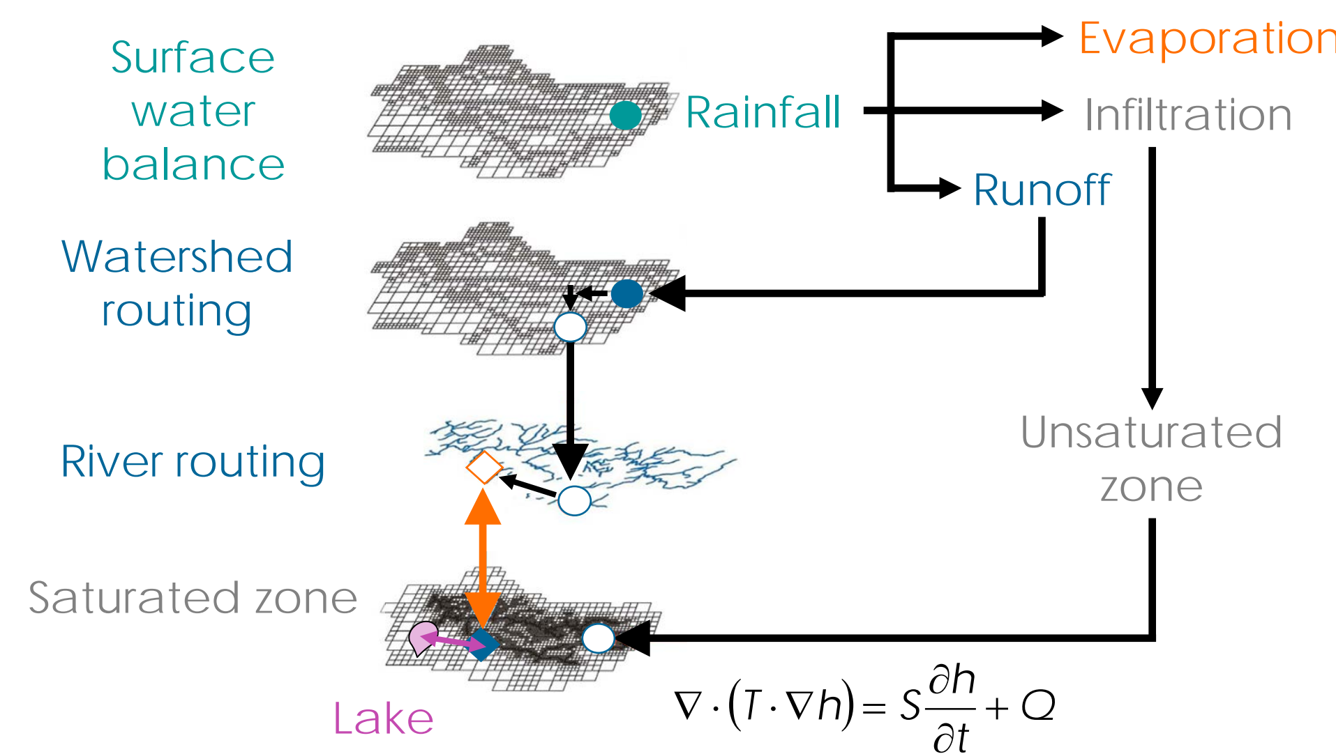
Fig. 3 – The EauDyssée platform for hydrosystem modeling
